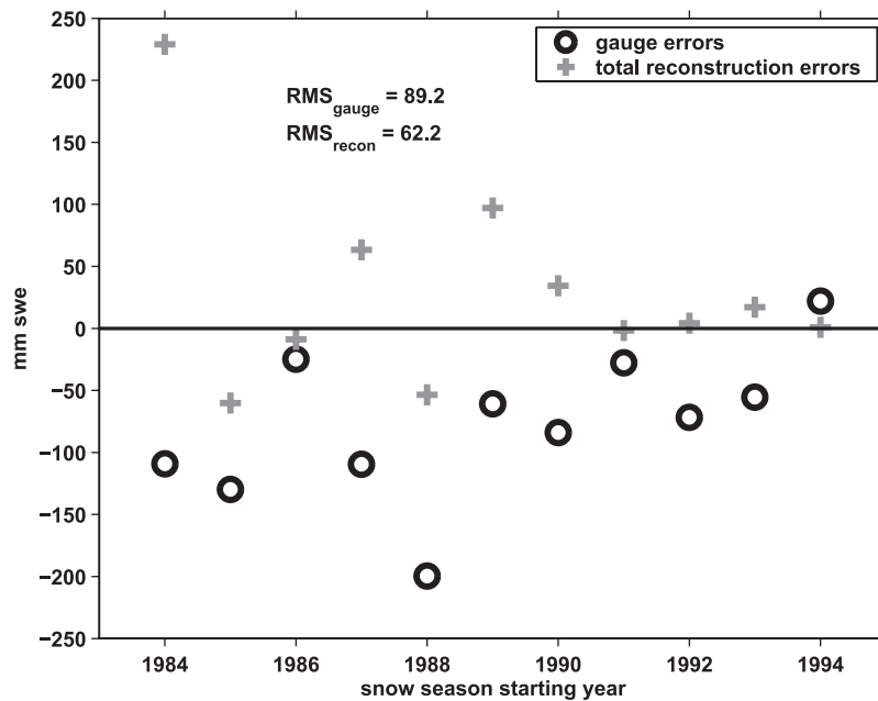
Figure 10. Cumulative errors from gauges (circles) and from the model (crosses) are averaged over the snow season of each year. The root-mean-square is calculated from this annual mean of cumulative error and is in units of millimeters SWE.
