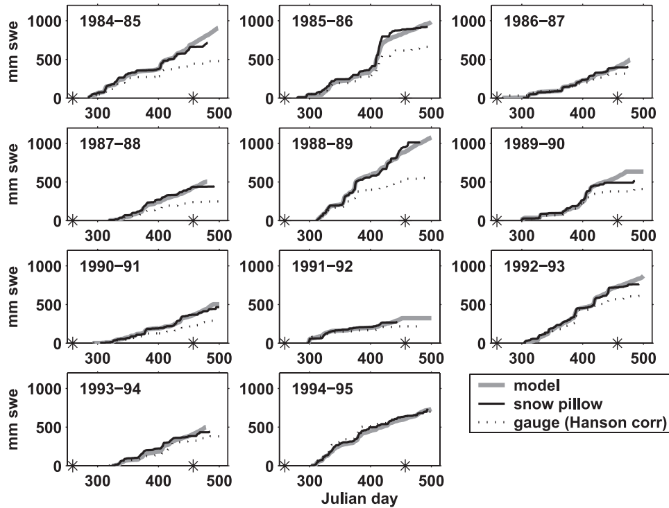
Figure 6. Cumulative snowfall is plotted with a thick line for a reconstruction (experiment 2) in which snow depth is restored to the control run, for the purpose of estimating errors. Observations from the snow pillow and the dual gauge with the Hanson correction are plotted with a thin line and a dashed line, respectively. Stars mark 15 September and 1 April, the period of reconstruction.
